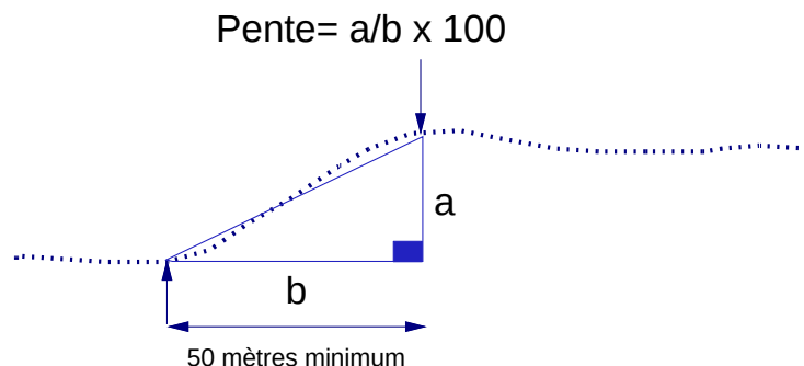
Figure 2.7d : Pente
